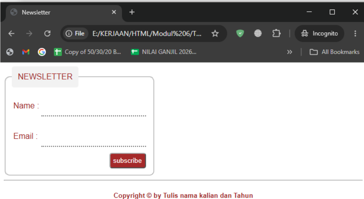
Gambar 1.4 Tampilan program 1.4
