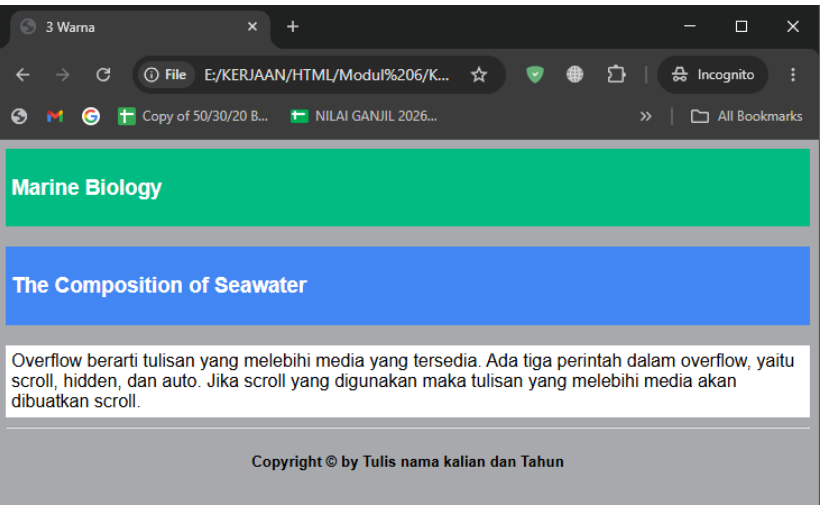
Gambar 1.3 Tampilan program 1.3
