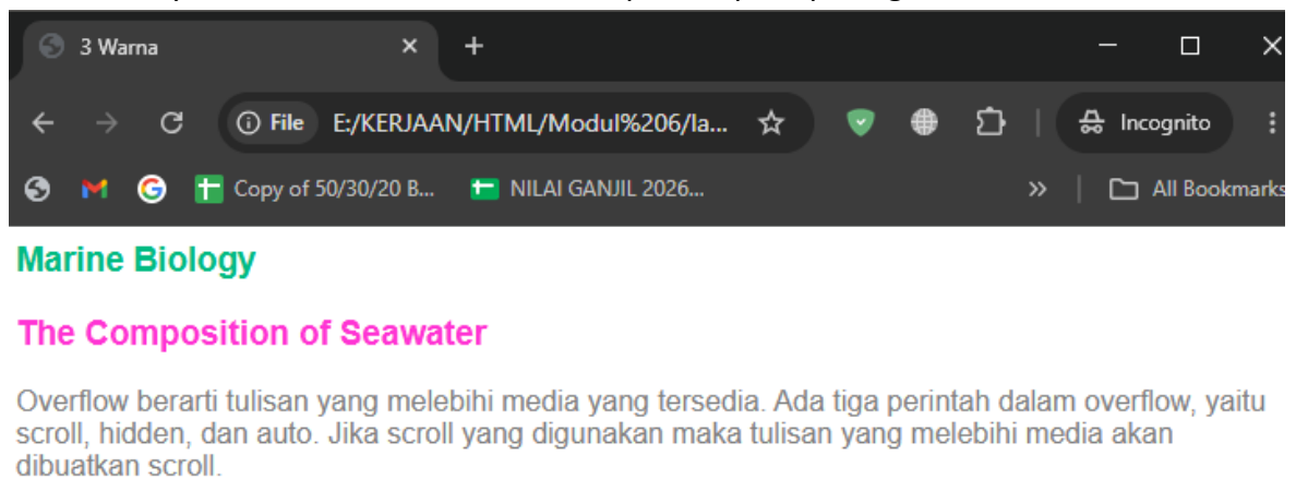
Gambar 1.2 Tampilan program 1.1
