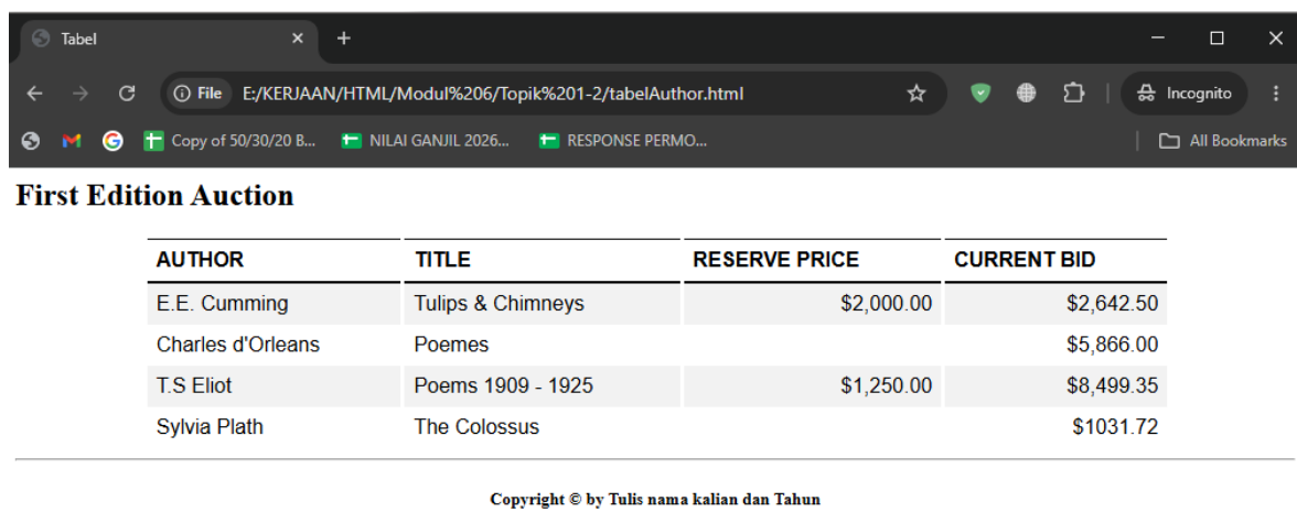
Gambar 1.5 Tampilan program 1.5
