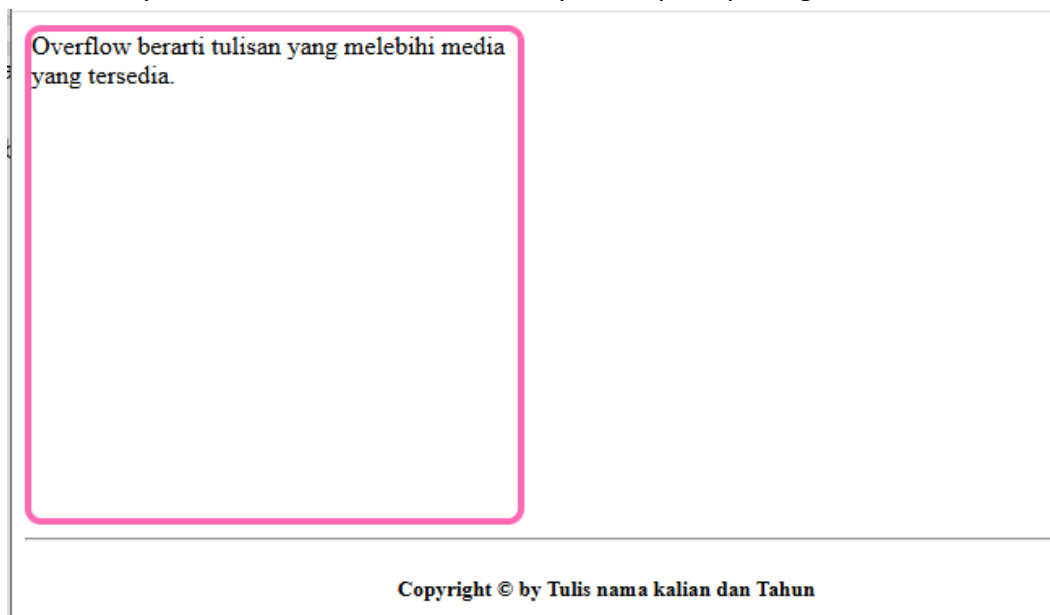
Gambar 1.1 Tampilan program 1.1
